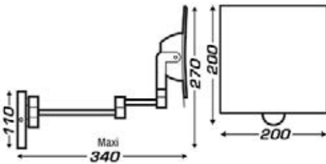
REF 8 66 769 Galaxy wall-mounted Brass chrome UPC 12
