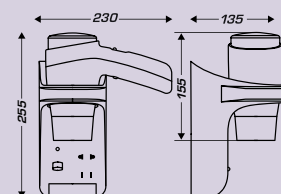
REF 8 22 407 Oceanis PR 1600W Black + wall-mounted holder + shaver unit UPC 12
