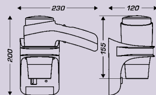
REF 8 22 413 Oceanis DC 1600W White + wall holder UPC 12
